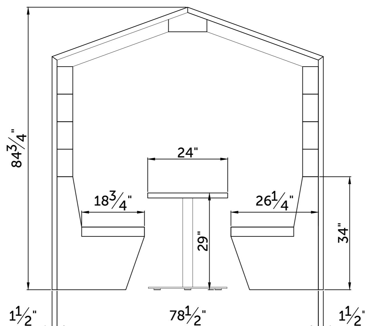
4 - Seater RWC Pitched roof Open
