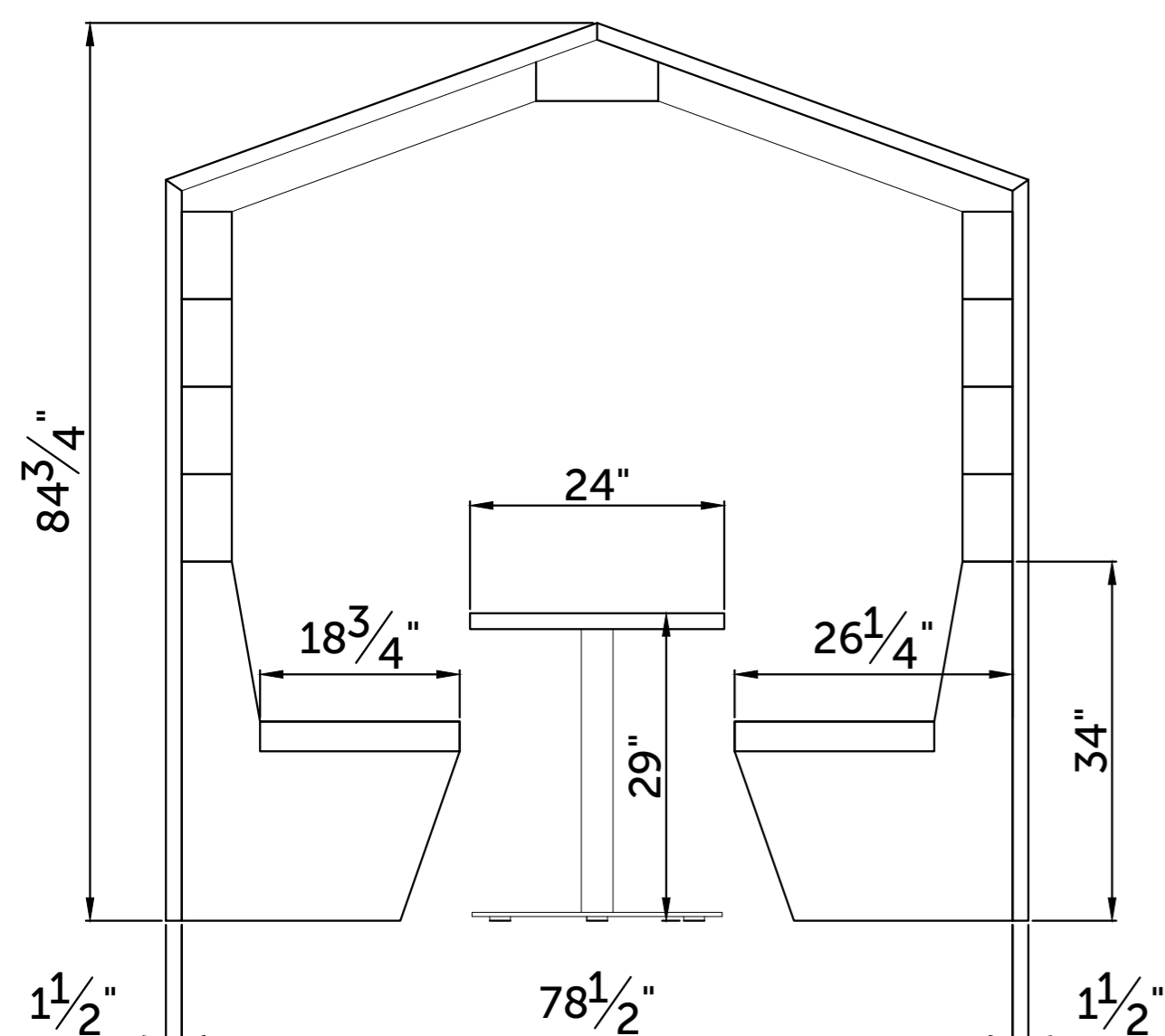
2 - Seater RWC Pitched roof Open
