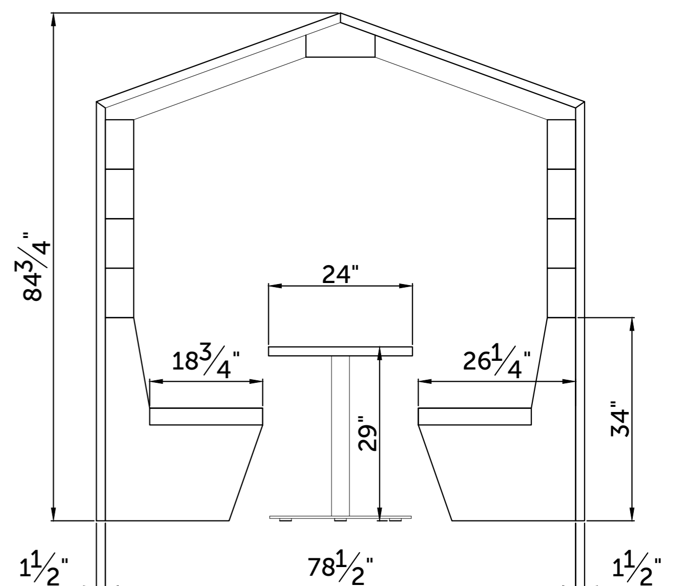
6 - Seater RWC Pitched roof (Square) Open
